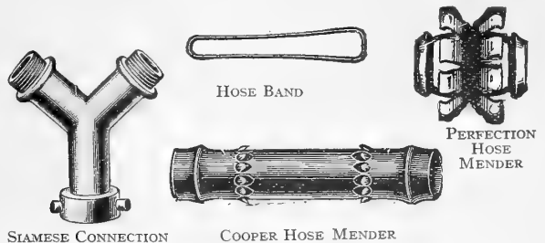
SIAMESE CONNECTION HOSE BAND COOPER HOSE MENDER PERFECTION HOSE MENDER
